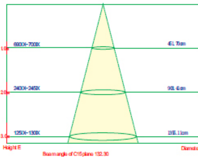
Lux distance curve(lux)
