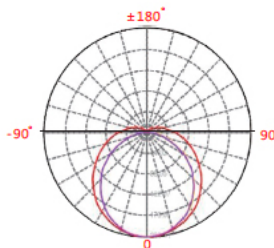
Light Distribution Curve(cd)
